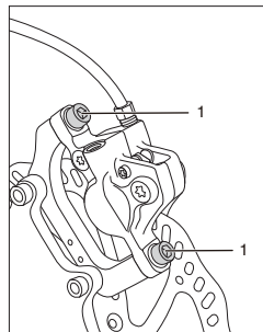
1. Alignment Bolts
